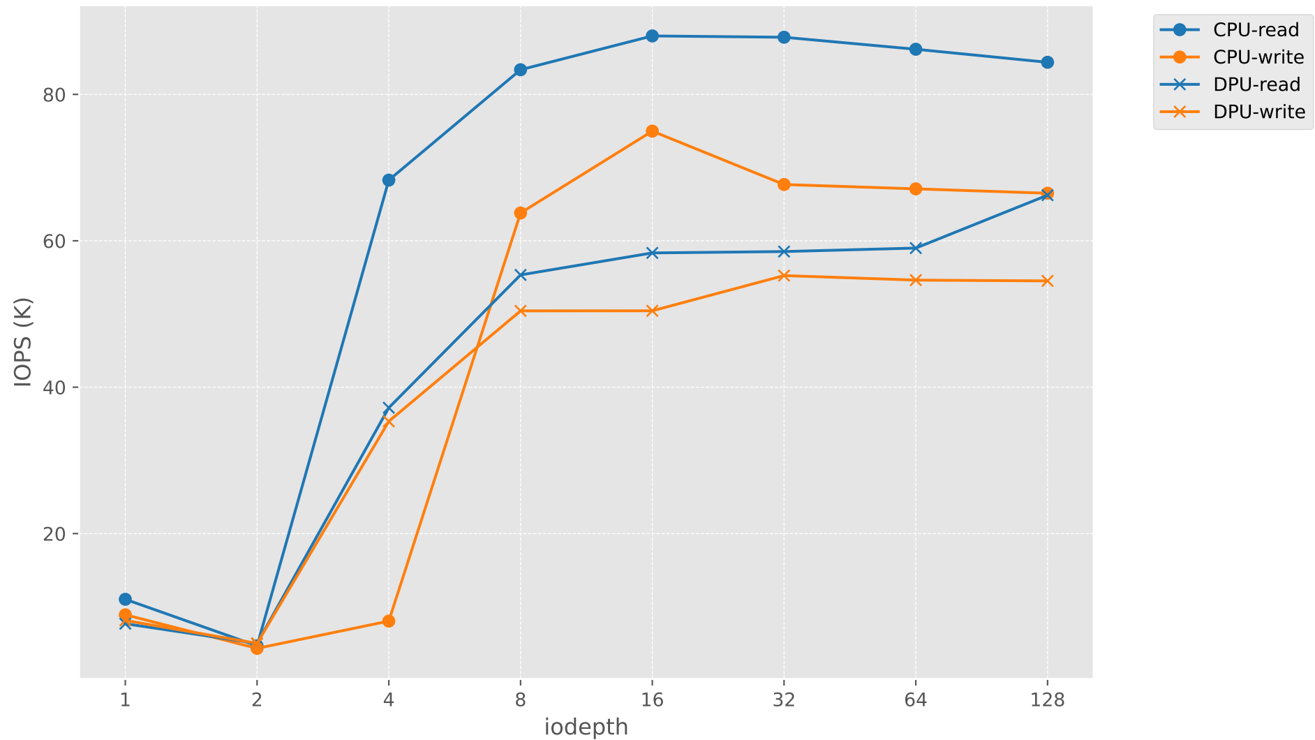
IOPS vs iodepth (Sequential)
